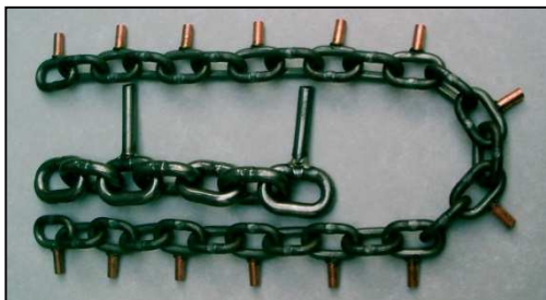
Link chains with welded on driver for special conveyor systems
