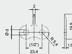
Design 112.10
