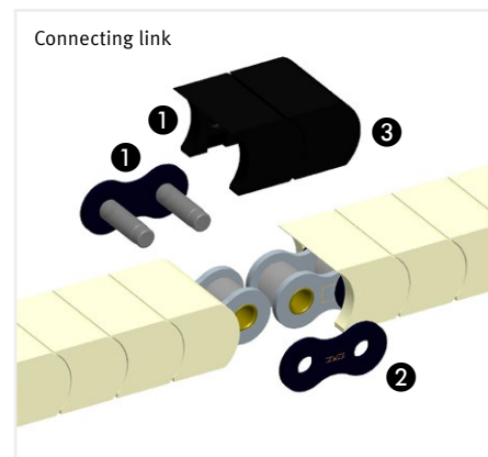
Connecting link: Same dimensions as chain
