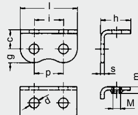
Design 203.2
