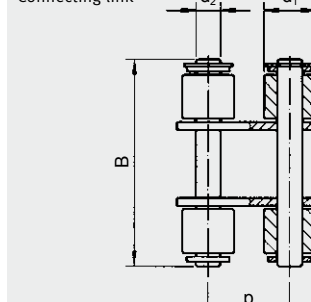
Connecting link
