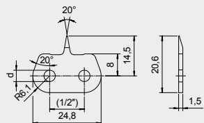
Design 112.06
