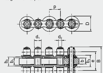
Design M normal pitch
