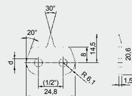
Design 112.09
