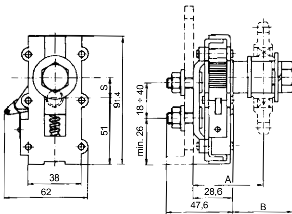
AMS 10
