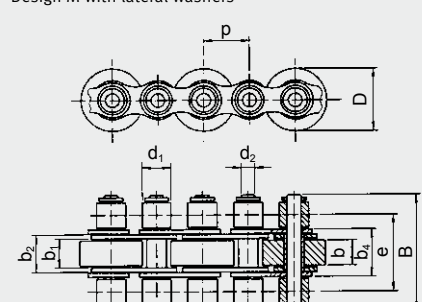
Design M with lateral washers
