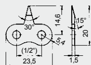
Design 112.0
