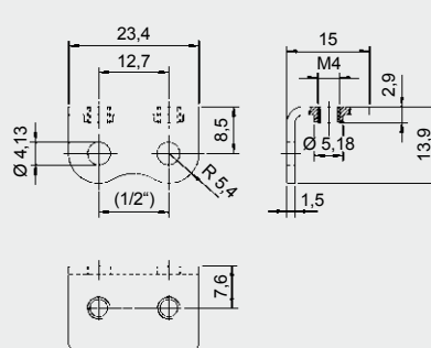
For chain L 85 SL: Design 203.32
