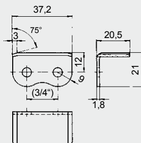
For chain M 127 SL: Design 203.8
