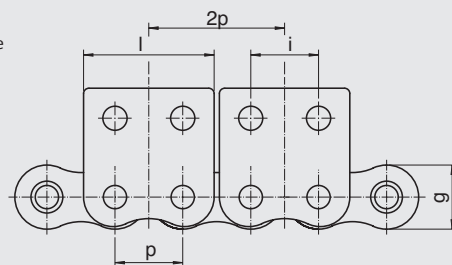
D2 Attachment plate on one side EC-1030.2
